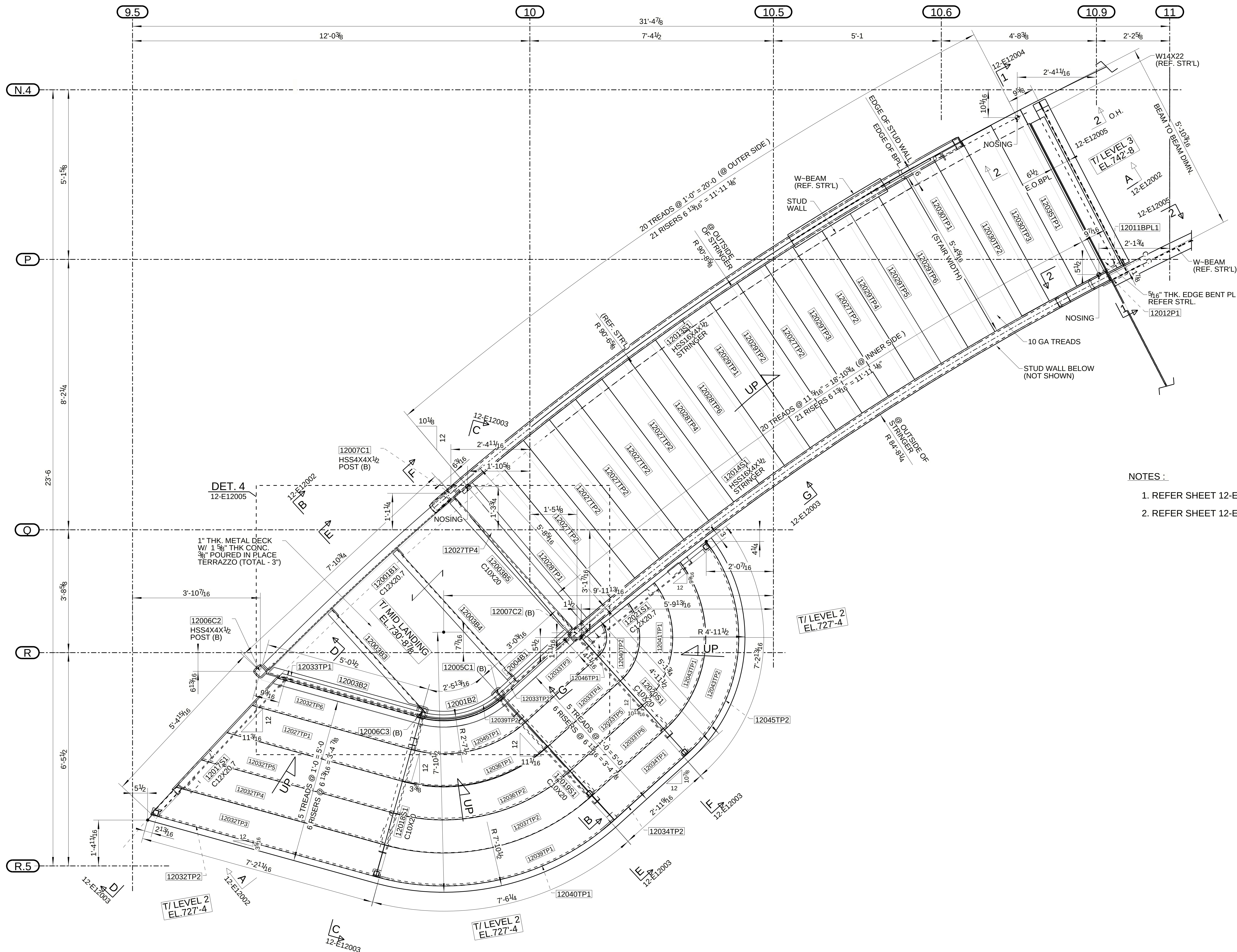
FRAMING PLAN FOR COMMON STAIR @ 2ND FLOOR (NORTH SIDE) (REFER : COMMON STAIR - ENLARGED PLAN - A13/A7.01)
