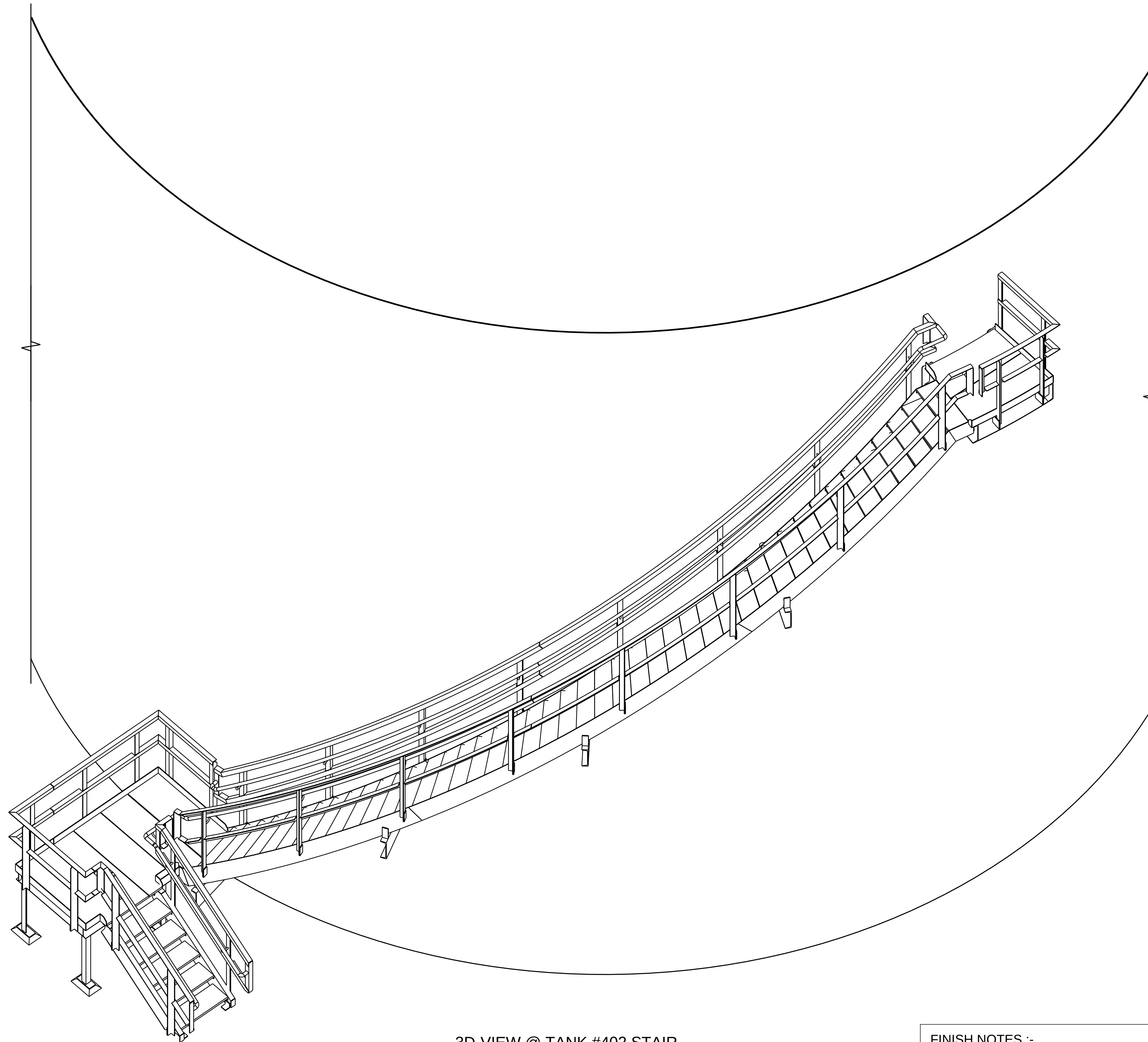
3D-VIEW @ TANK #402 STAIR
