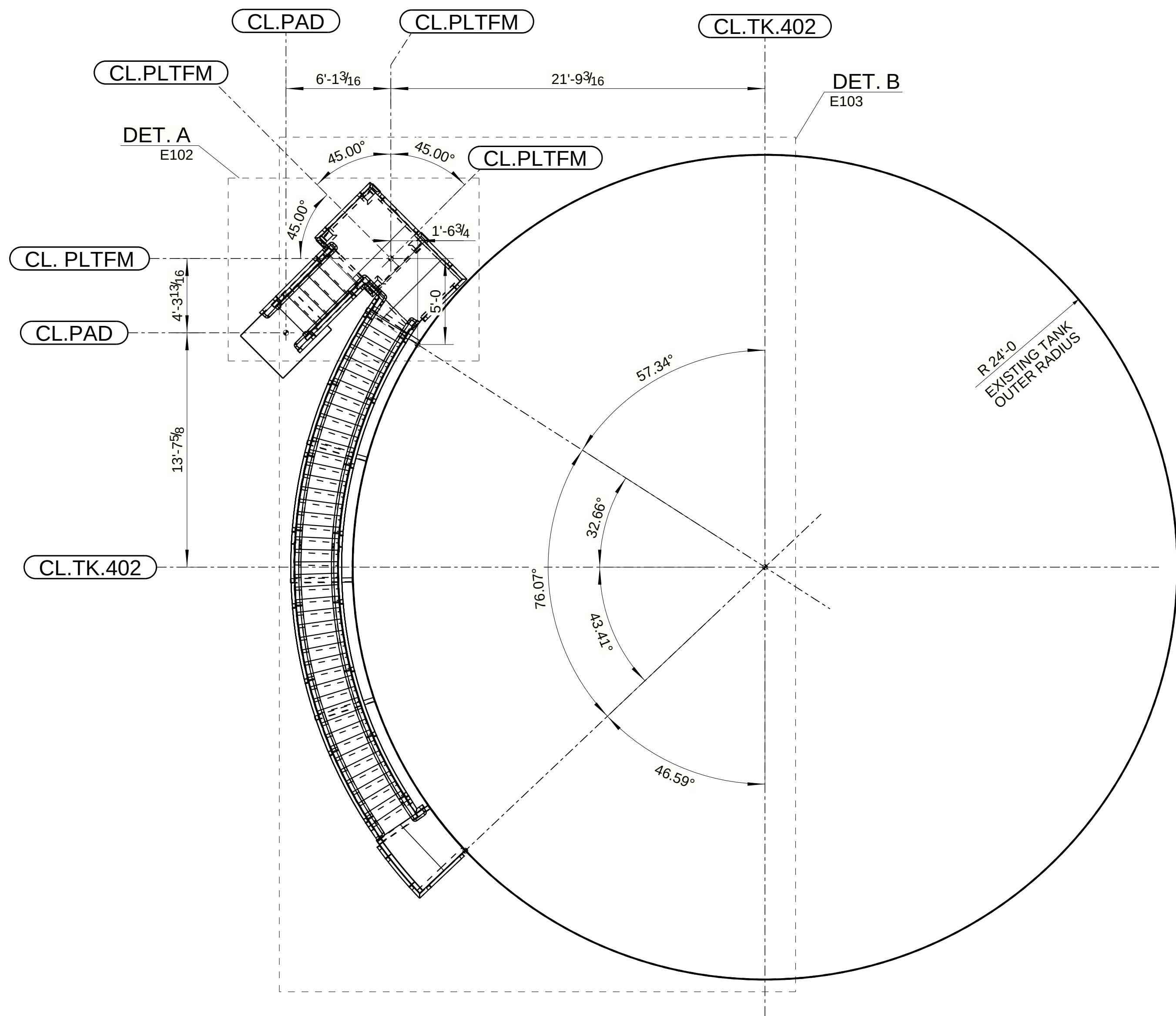
TK 402 STAIR LOCATION PLAN (REFER : TK 402 STAIR LOCATION PLAN / D-400-3003-21)
