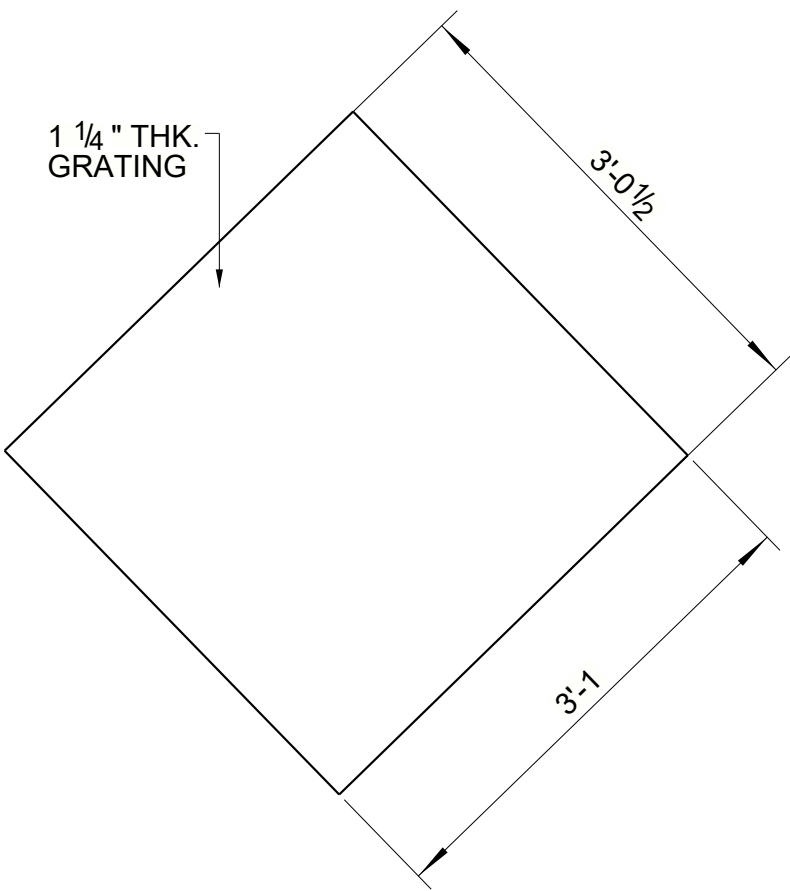
TYPICAL LANDING GRATING LAYOUT PLAN @ LANDING 01, 02, 03, 04, 05, 06
