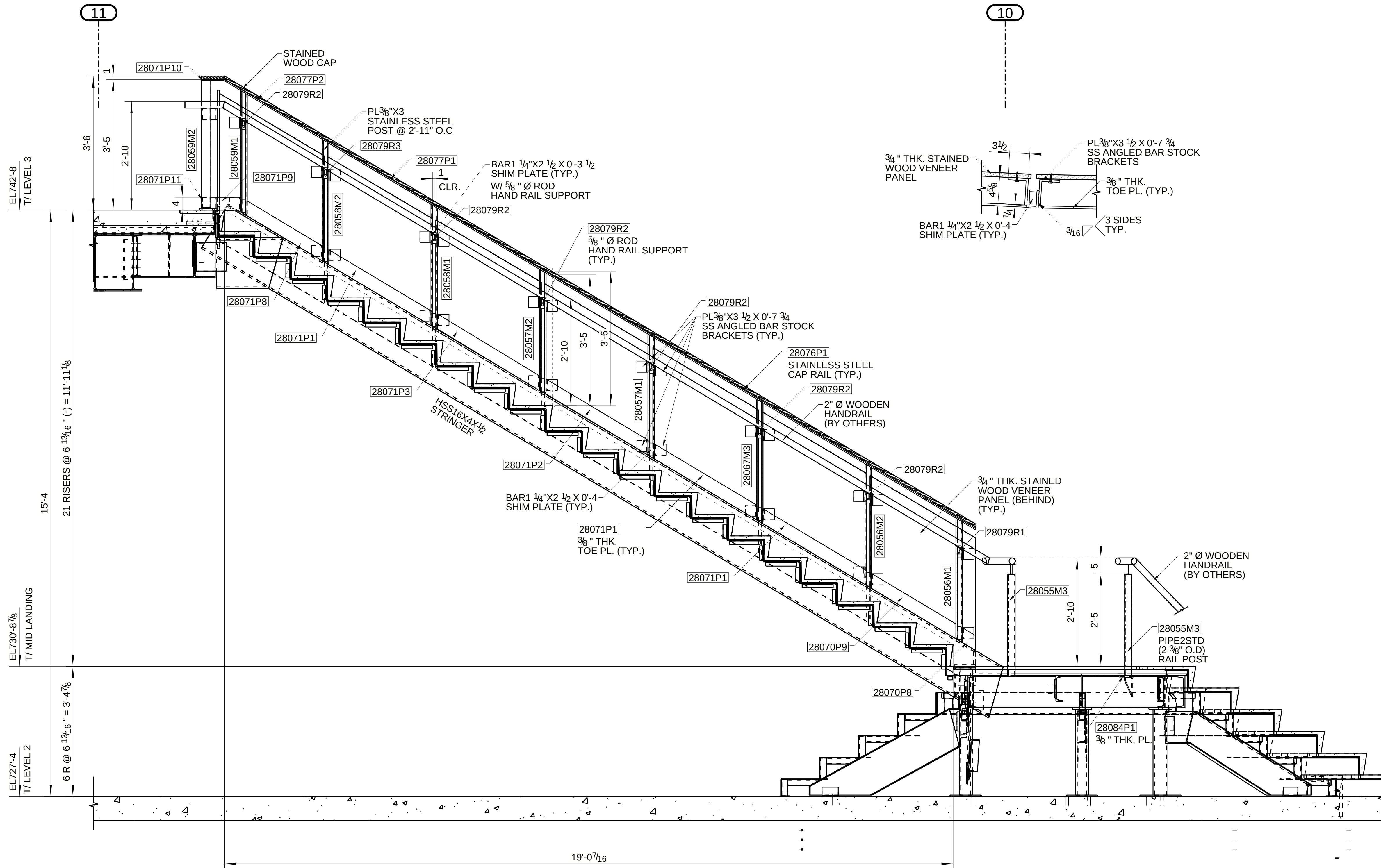
SECTION B - B 28-E28031
