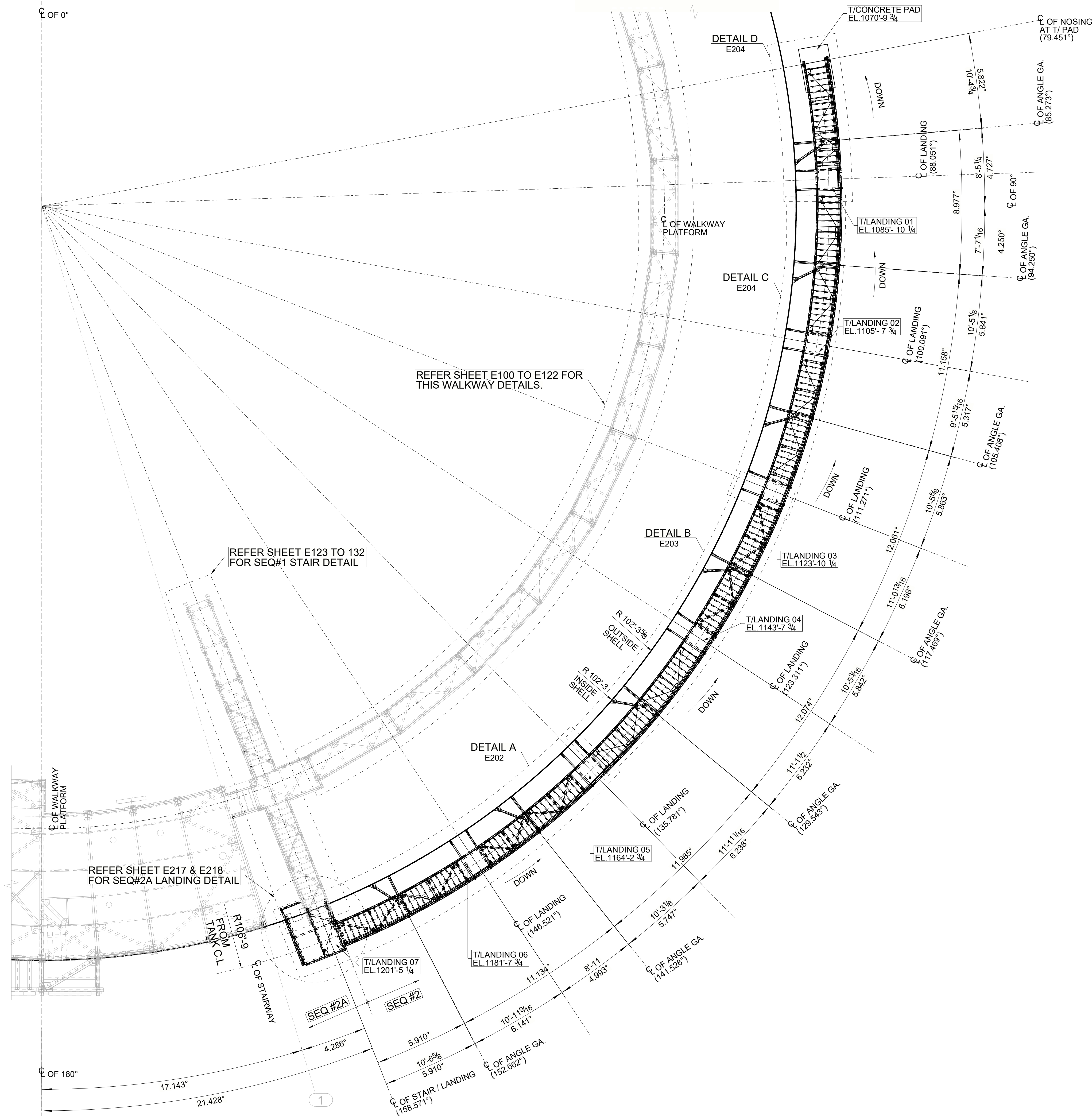
SEQ#2 SPIRAL STAIR KEY PLAN (REFER : PLAN OF SPIRAL STAIRWAY /DW-10600-01)
